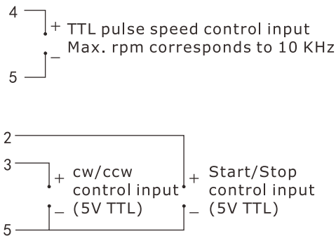
Pulse Input External Control Module Wiring Diagram
